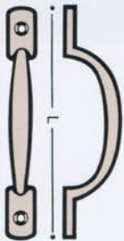
1436 SASH HANDLE lengths L : 102, 127, 152
