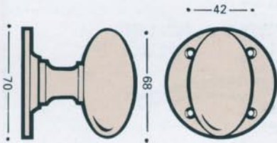
1016 OVAL KNOB
