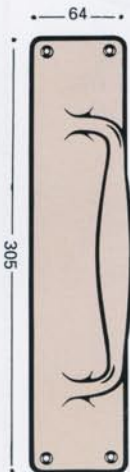
1440 PULL HANDLE • face fixed • rear bolt fixing available upon request
