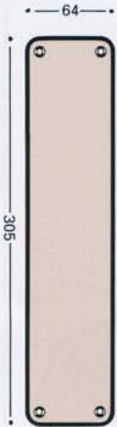
1440 FINGER PLATE • solid cast • designed to match 1440 pull handle
