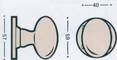
1021 OVAL KNOB 2999 C/W MICROTITE SPINDLE
