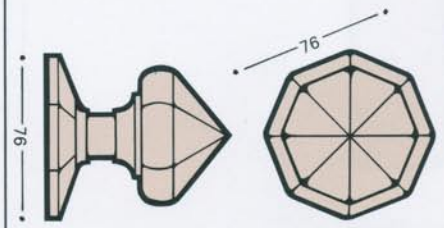
1068CDK CENTRE DOOR KNOB • octagonal design
