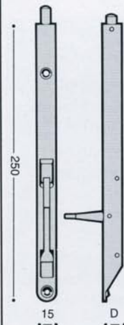
5650 BOLT • lever action • made from corrosion free stainless steel • available in satin or polished finish • smooth easy action • round ends shoot size : 7.5 diameter length of throw : 16 depth of mortice D : 15
