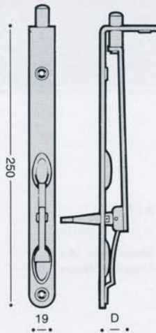
5654 BOLT • lever action • made from corrosion free stainless steel • available in satin or polished finish • smooth easy action • round ends shoot size : 10 diameter length of throw : 17 depth of mortice D : 24
