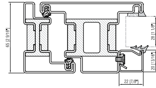
DOOR open out interior glazing bead
