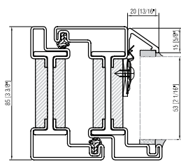
WINDOW open out exterior glazing bead
