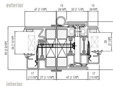
OS2 FXD mullied to OS2 CSMT with structural support inside the profile
