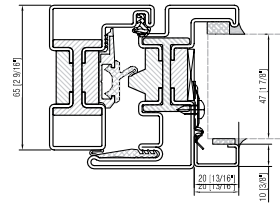
WINDOW open in interior glazing bead
