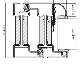
WINDOW open out exterior glazing bead
