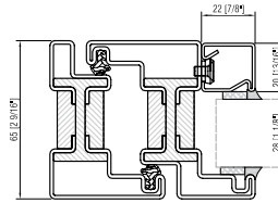
WINDOW open out exterior glazing bead
