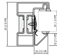
FIXED FRAME interior glazing bead
