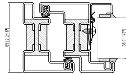
WINDOW open out exterior glazing bead
