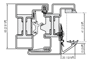
WINDOW open in interior glazing bead
