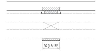
THINNER FLAT SDL
