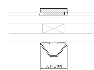
STANDARD STEEL SLOPED SDL
