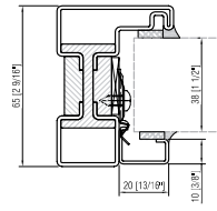
FIXED FRAME interior glazing bead
