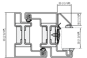
WINDOW open out exterior glazing bead
