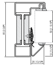
FIXED FRAME interior glazing bead
