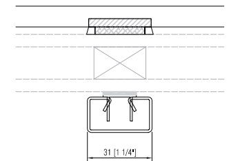
STANDARD SQUARE SDL
