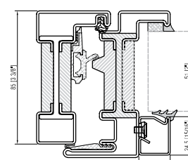
WINDOW open in interior glazing bead
