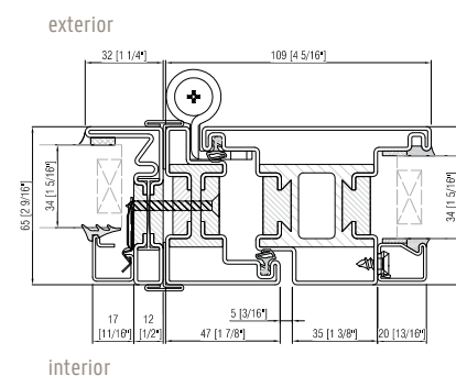
OS2 FXD mullied to EBE Hinged Door
